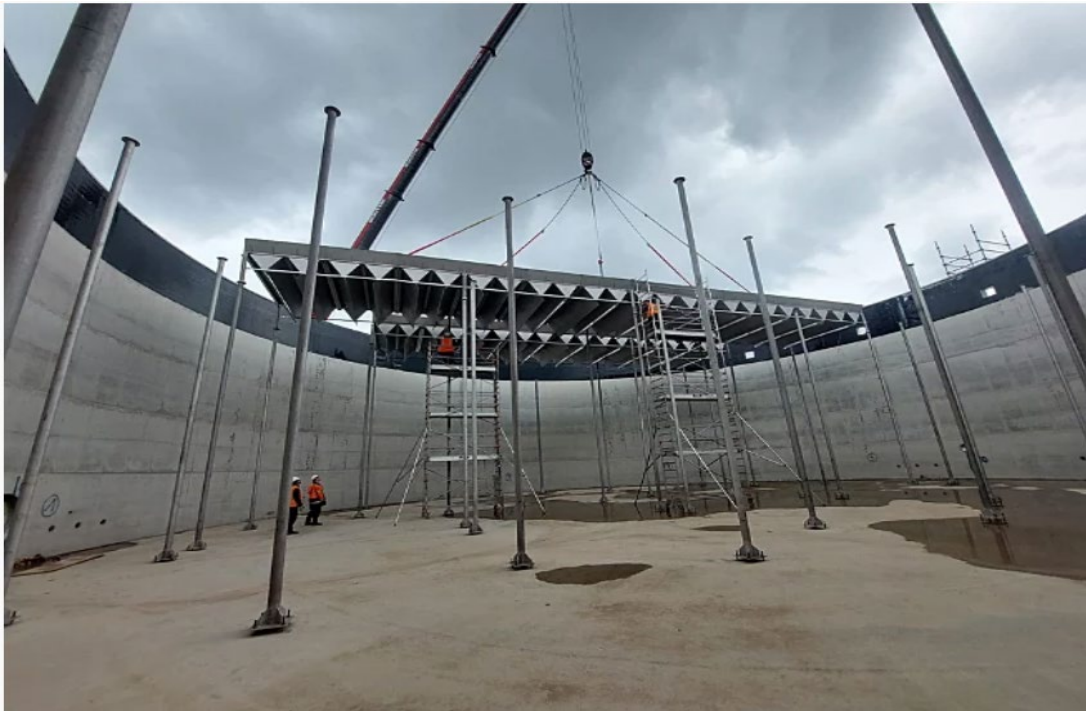
BIOTIM UASB under construction
